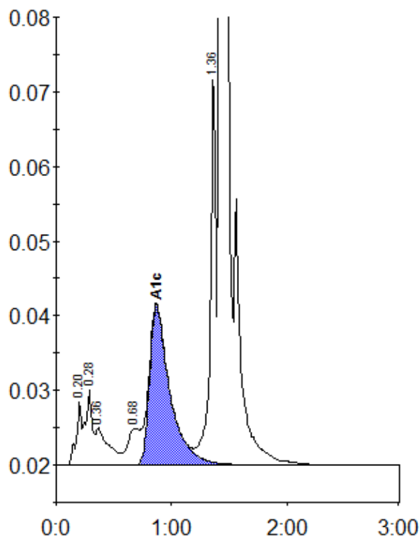
Peak table - ID: 10667889
